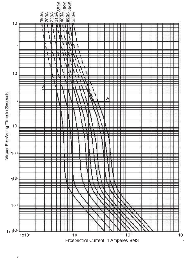
Size 1 — 160-630A: 1250V Time-Current Curve
